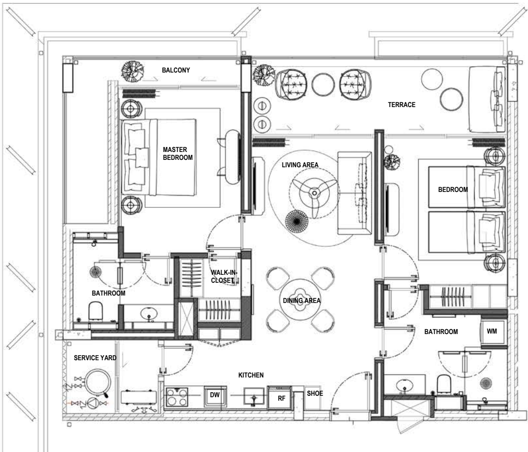
2 Bedroom Residence, Type 1
