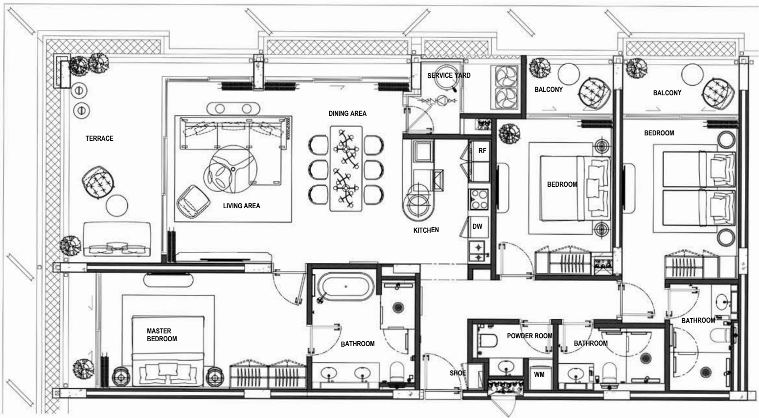
3 Bedroom Residence, Type 3
