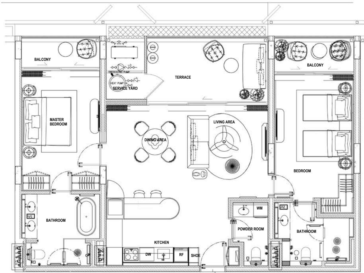
2 Bedroom Residence, Type 2
