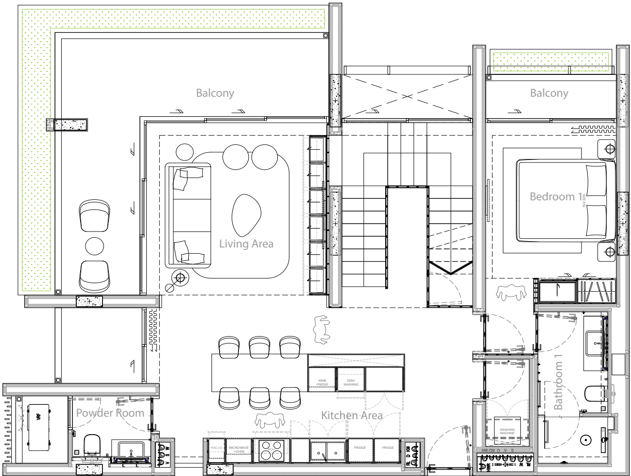
Lower Floor
