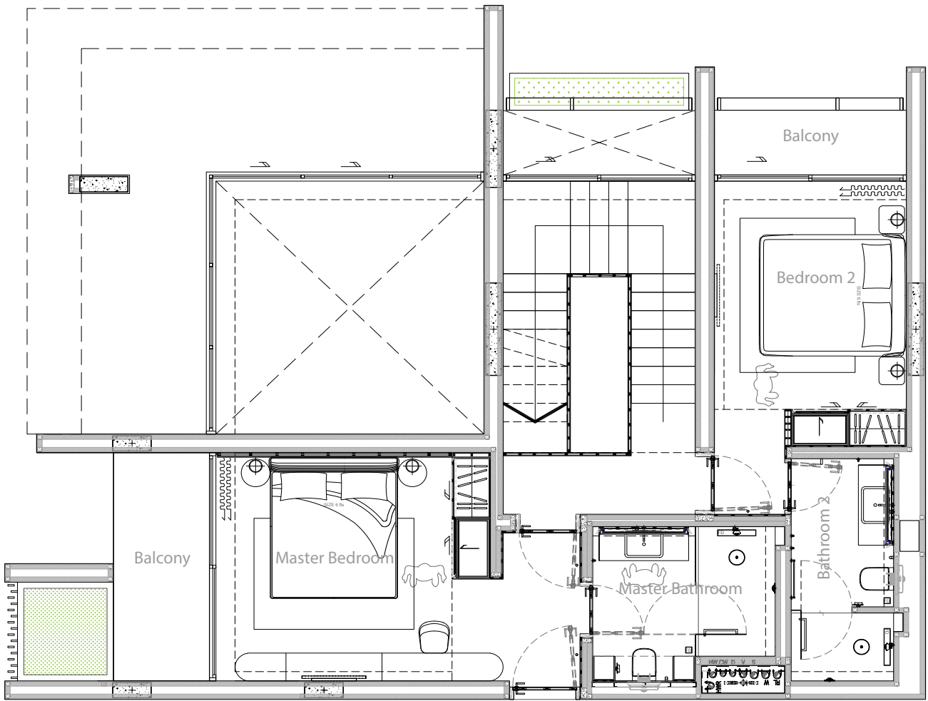
Upper Floor
